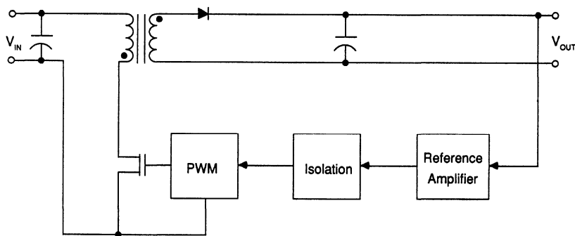
FIGURE 2. The Flyback Converter.
