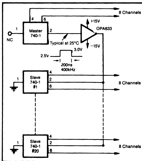
FIGURE 1. Master/Slave Synchronization of Multiple PWS740 Drivers.
