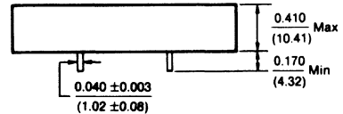
Side View—"A" Package Option
