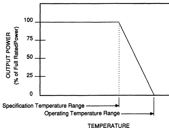
FIGURE 1. Derating Curve.
