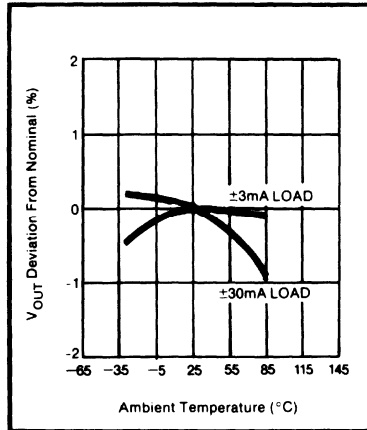
FIGURE 2. Temperature Drift.
