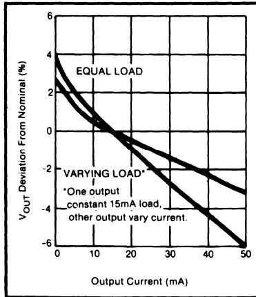
FIGURE 1. Load Regulation.
