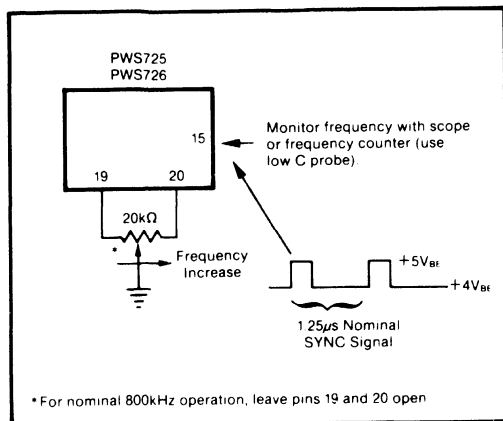
FIGURE 4. Frequency Adjustment Procedure.
