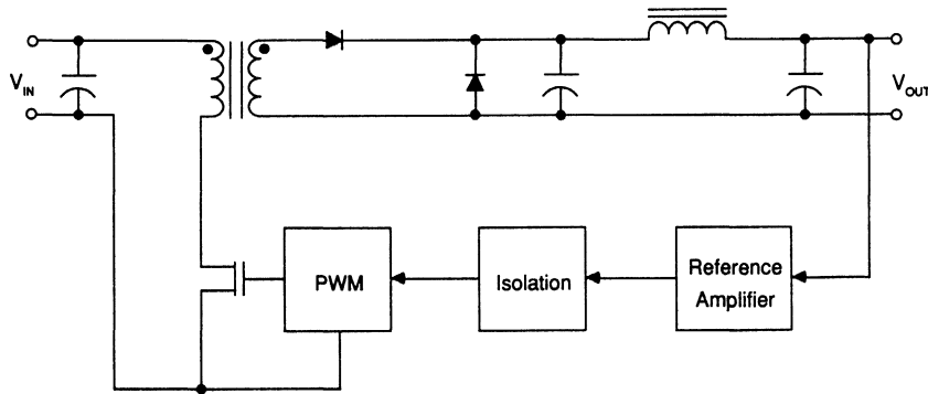
FIGURE 3. The Forward Converter (With Output PI Filter).
