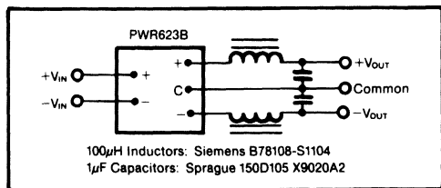
FIGURE 6. Filter Circuit for DC/DC Converter.
