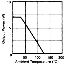
POWER DERATING
