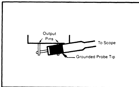
FIGURE 1. Recommended Noise Measurement Method.
