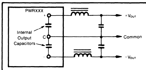
FIGURE 2. Output "PI" Filters.
